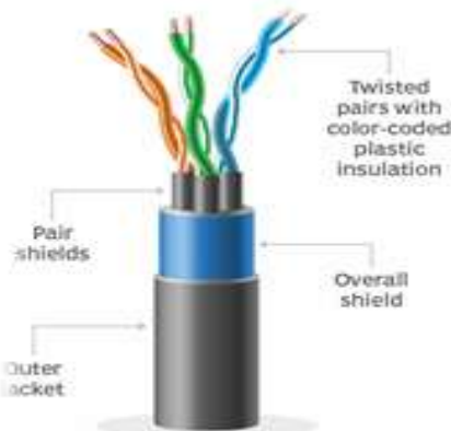
Shielded twisted pair
